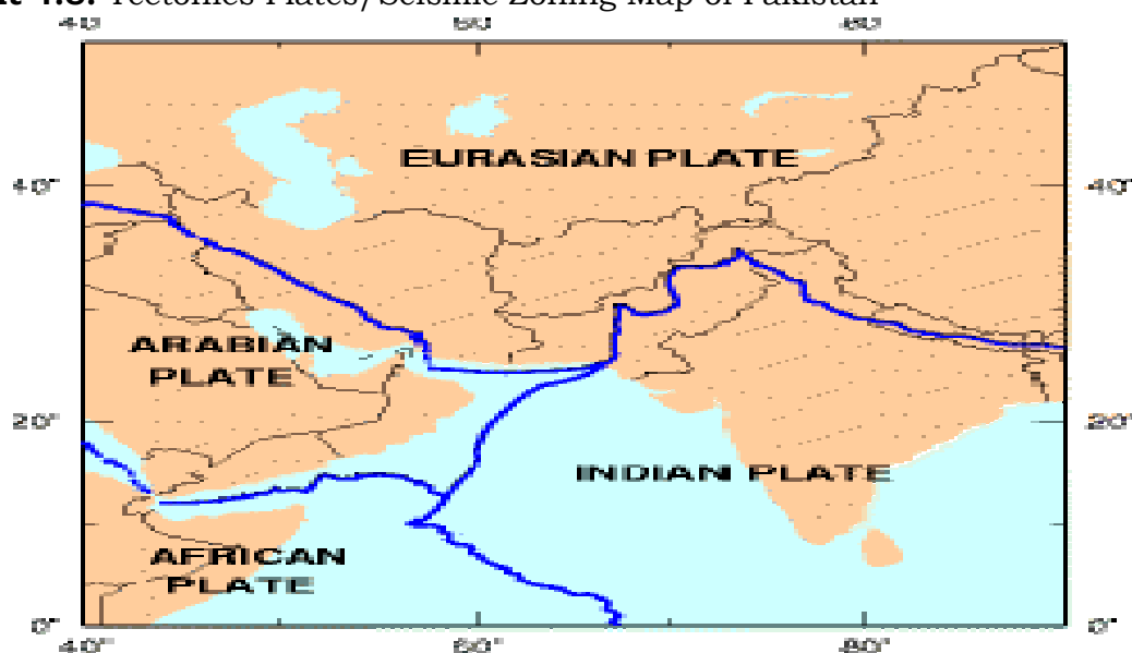
Exhibit 4.8: Tectonics Plates/Seismic Zoning Map of Pakistan
