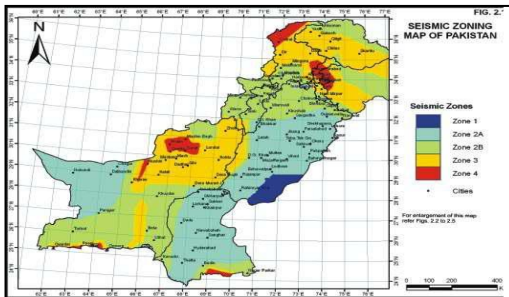
Exhibit 4.9: Karachi lies on 2B Seismic Zone
