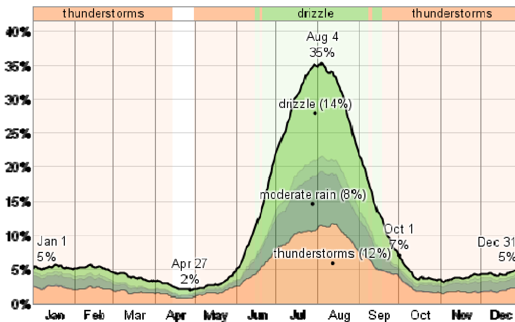
Exhibit 4.3: Mean monthly precipitation for Karachi south District
