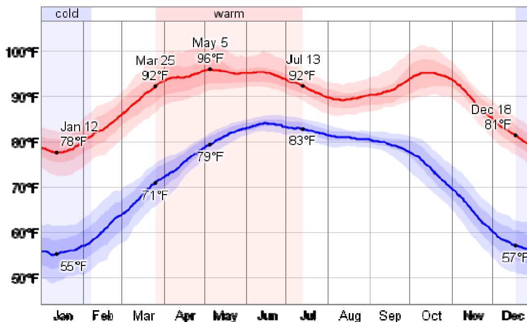
Exhibit 4.2: Yearly mean and minimum temperature
